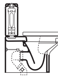
INODORO COMPACTO TANQUE BAJO BTW Close-coupled compact WC suite with dual trap
